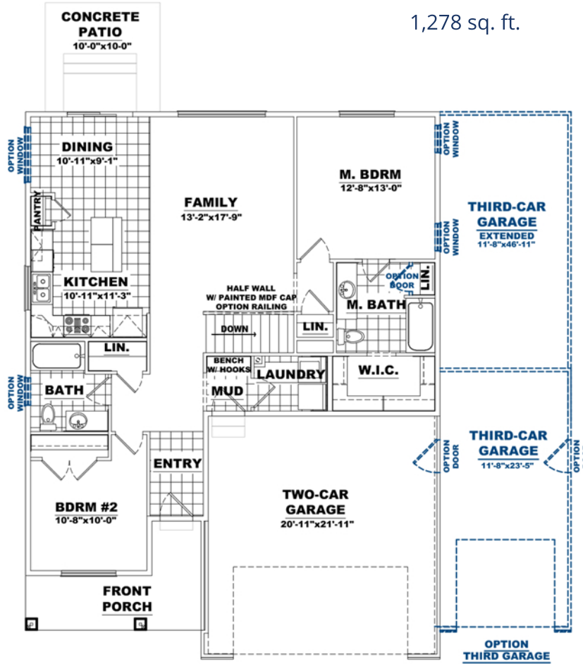
MAIN LEVEL
