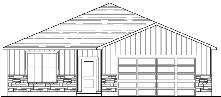
FARMHOUSE ELEVATION
