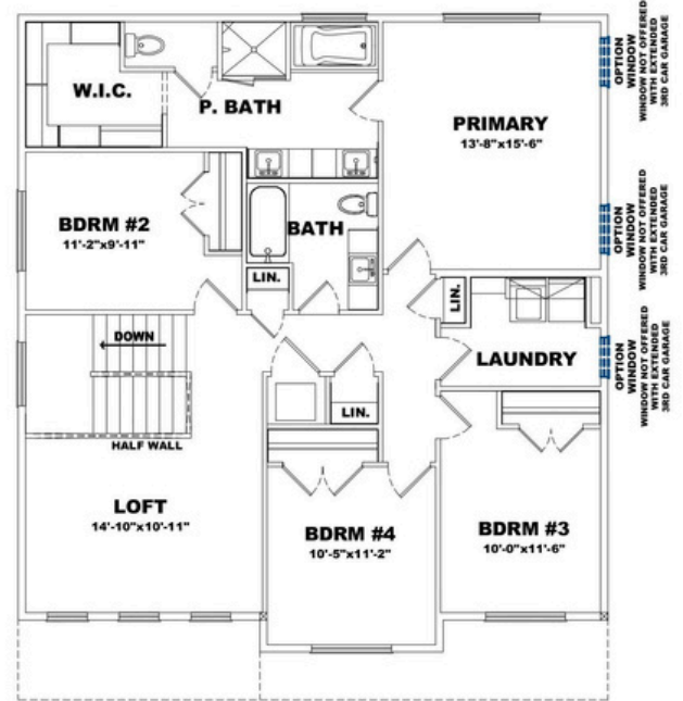
SECOND LEVEL
