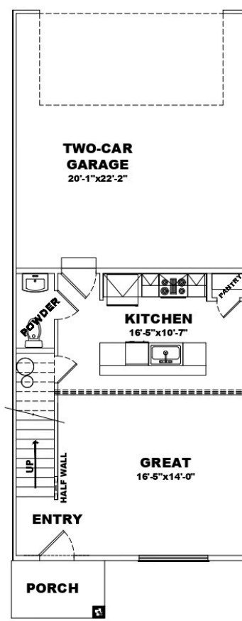
MAIN LEVEL
