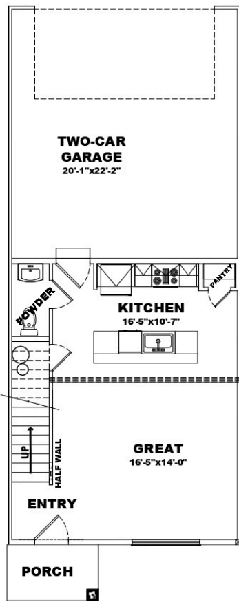
MAIN LEVEL
