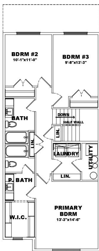
SECOND LEVEL
